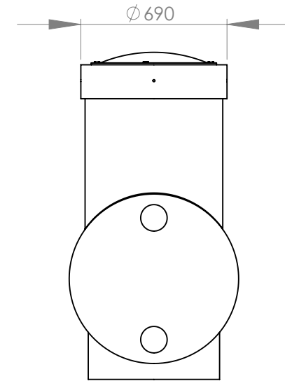
END VIEW
